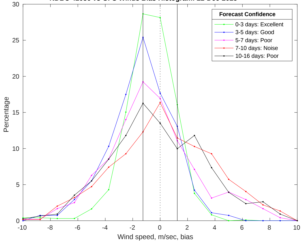
NDBC 42036 vs GFS Winds Bias Histogram: 22-Dec-2025
