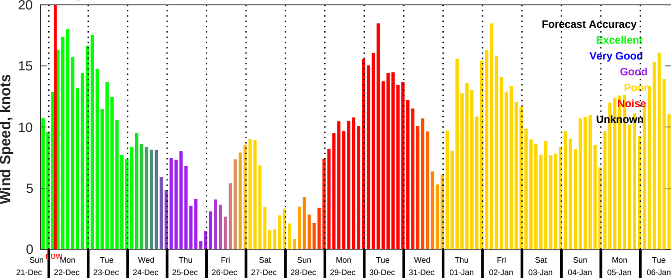
GFS Wind Speed Forecast for NDBC 42036 from 21-Dec-2025 19:00:00 to 06-Jan-2026 19:00:00
