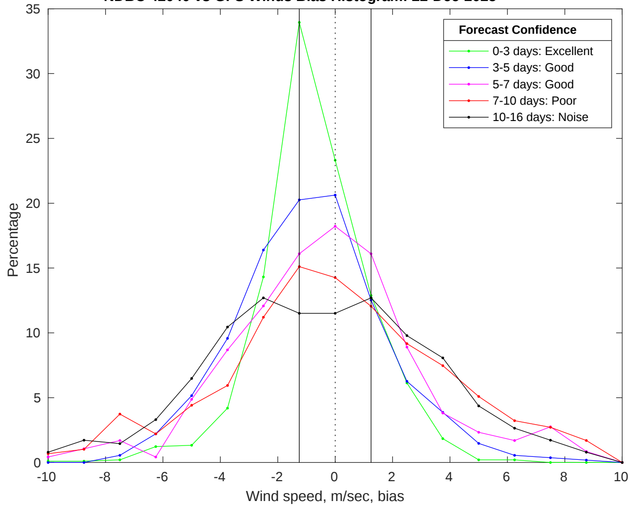
NDBC 42040 vs GFS Winds Bias Histogram: 22-Dec-2025
