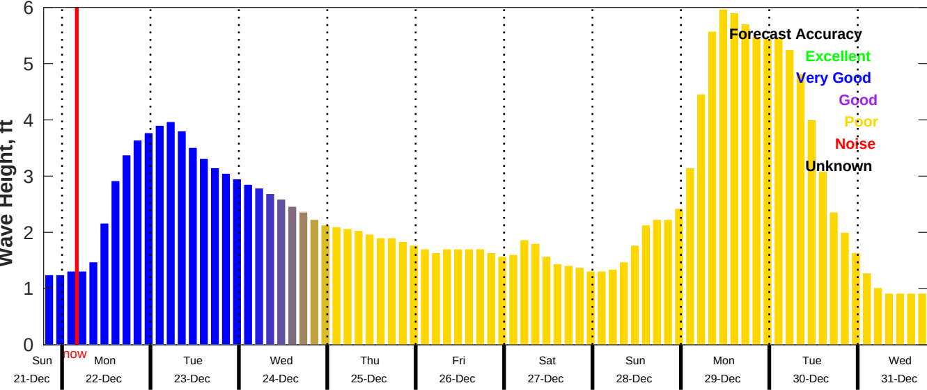
CMEMS Wave Forecast for NDBC 42040 from 21-Dec-2025 19:00:00 to 31-Dec-2025 19:00:00
