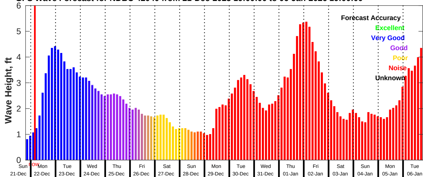
GFS Wave Forecast for NDBC 42040 from 21-Dec-2025 19:00:00 to 06-Jan-2026 19:00:00
