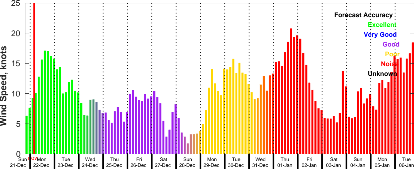
GFS Wind Speed Forecast for NDBC 42040 from 21-Dec-2025 19:00:00 to 06-Jan-2026 19:00:00
