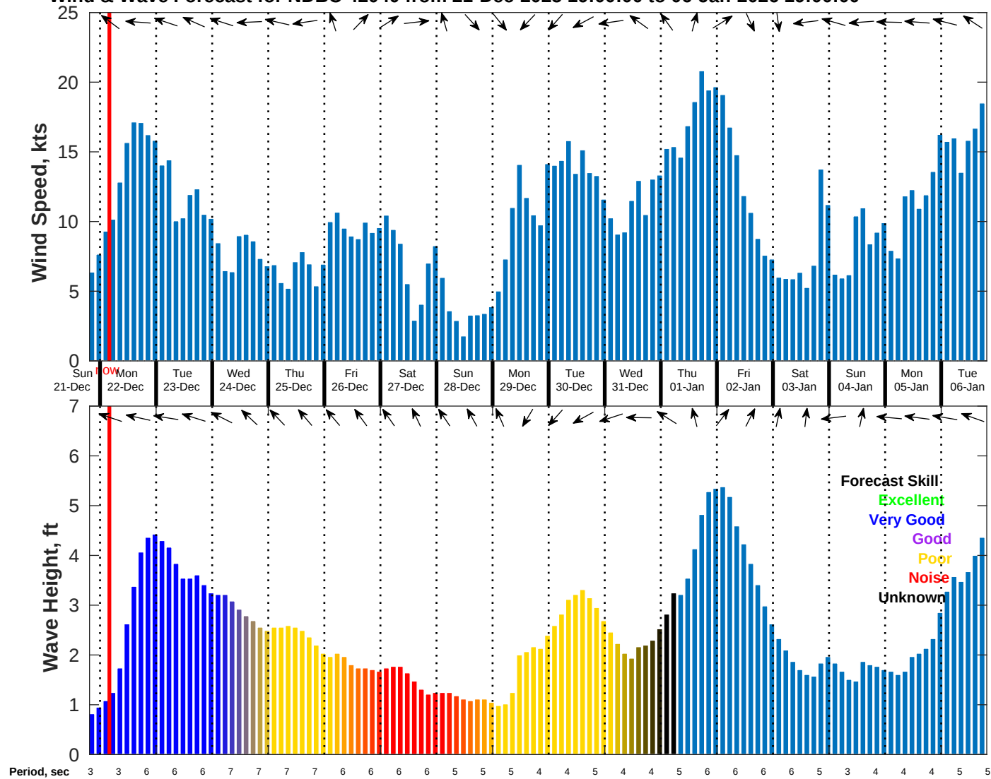
Wind & Wave Forecast for NDBC 42040 from 21-Dec-2025 19:00:00 to 06-Jan-2026 19:00:00
