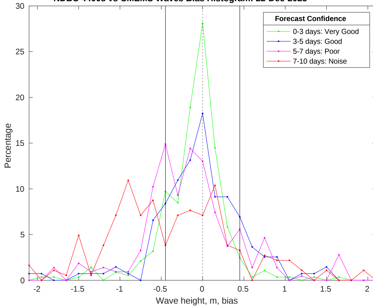
NDBC 44008 vs CMEMS Waves Bias Histogram: 22-Dec-2025
