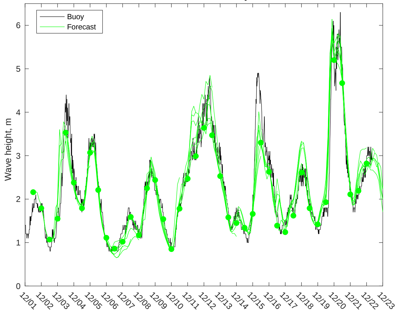
NDBC 44008 vs GFS Waves: 0 to 3 day forecast
