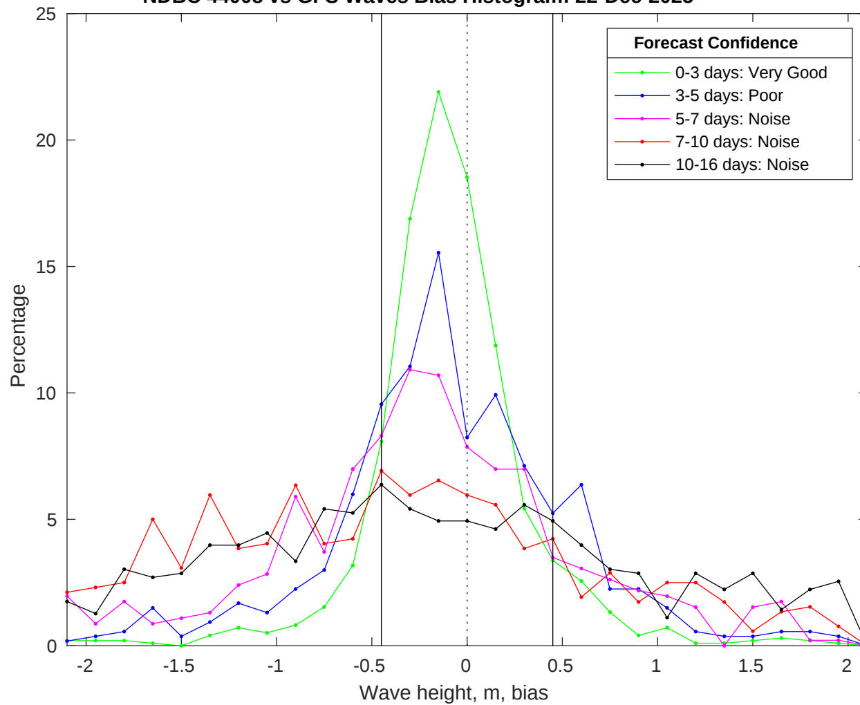
NDBC 44008 vs GFS Waves Bias Histogram: 22-Dec-2025
