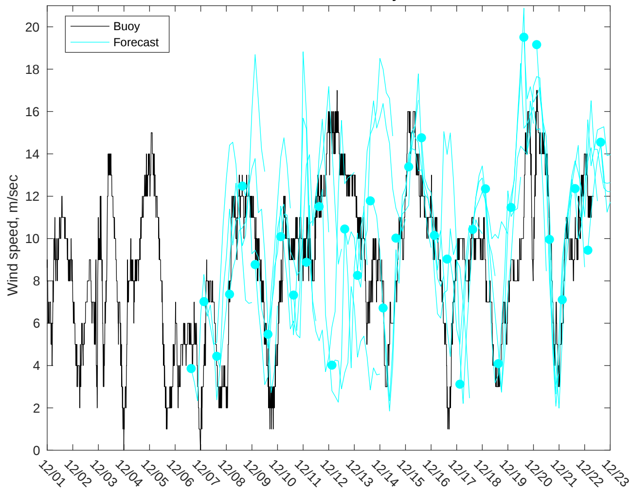
NDBC 44008 vs GFS Winds: 5 to 7 day forecast
