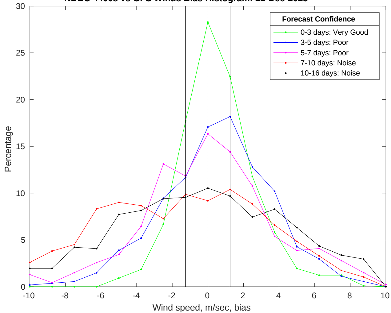
NDBC 44008 vs GFS Winds Bias Histogram: 22-Dec-2025
