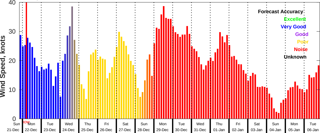
GFS Wind Speed Forecast for NDBC 44008 from 21-Dec-2025 20:00:00 to 06-Jan-2026 20:00:00
