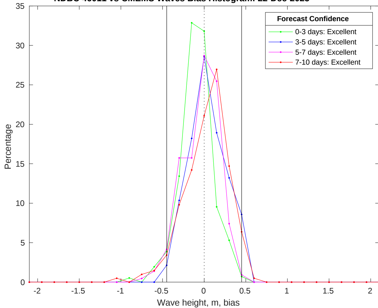
NDBC 46011 vs CMEMS Waves Bias Histogram: 22-Dec-2025
