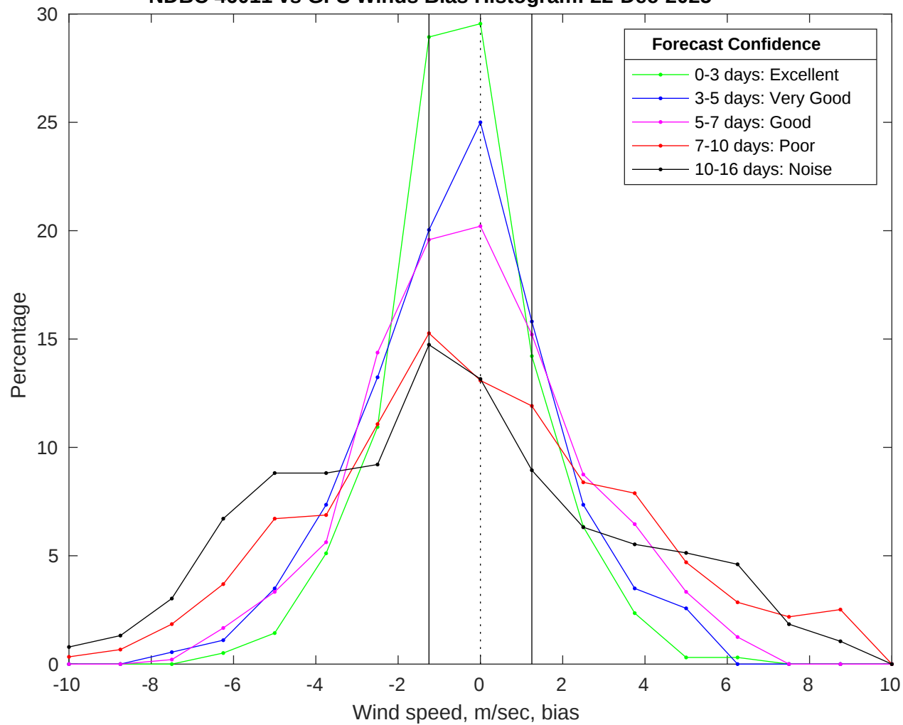
NDBC 46011 vs GFS Winds Bias Histogram: 22-Dec-2025
