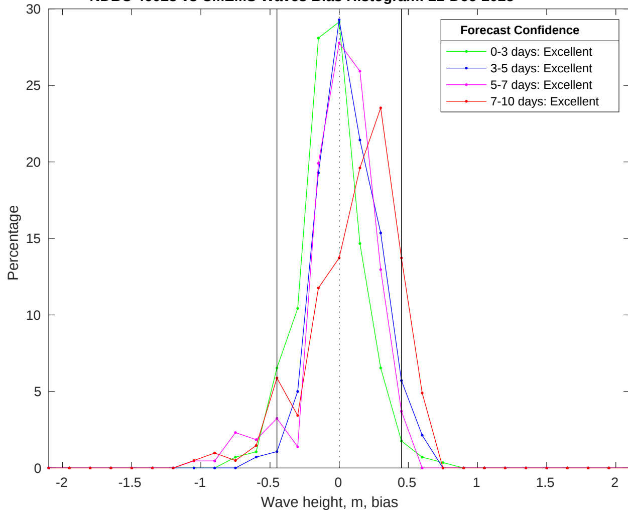
NDBC 46028 vs CMEMS Waves Bias Histogram: 22-Dec-2025
