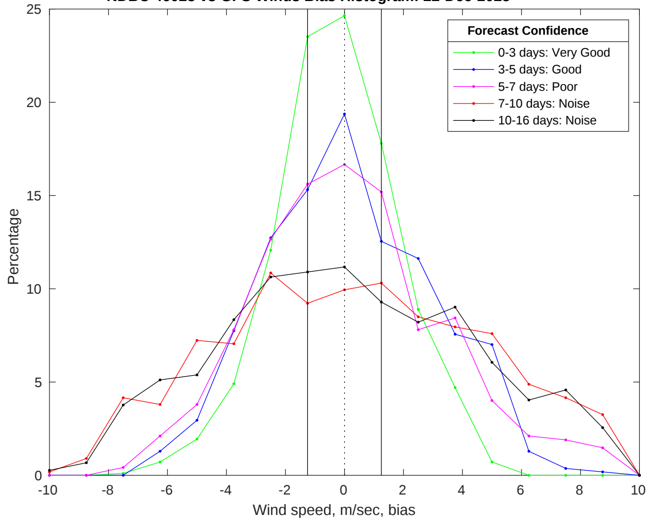
NDBC 46028 vs GFS Winds Bias Histogram: 22-Dec-2025
