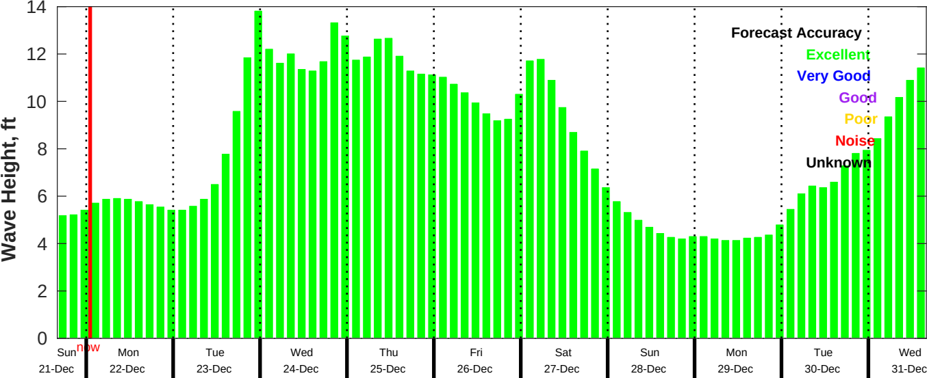
CMEMS Wave Forecast for NDBC 46028 from 21-Dec-2025 16:00:00 to 31-Dec-2025 16:00:00
