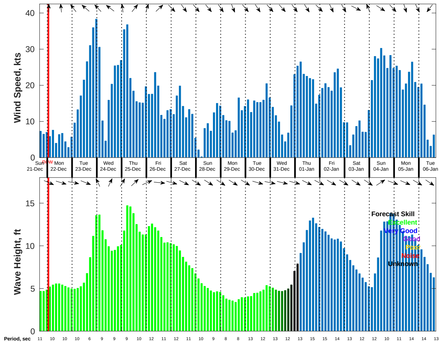
Wind & Wave Forecast for NDBC 46028 from 21-Dec-2025 16:00:00 to 06-Jan-2026 16:00:00
