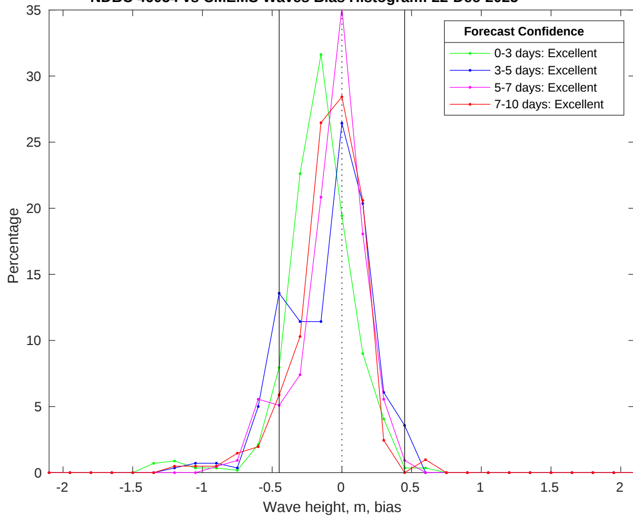
NDBC 46054 vs CMEMS Waves Bias Histogram: 22-Dec-2025
