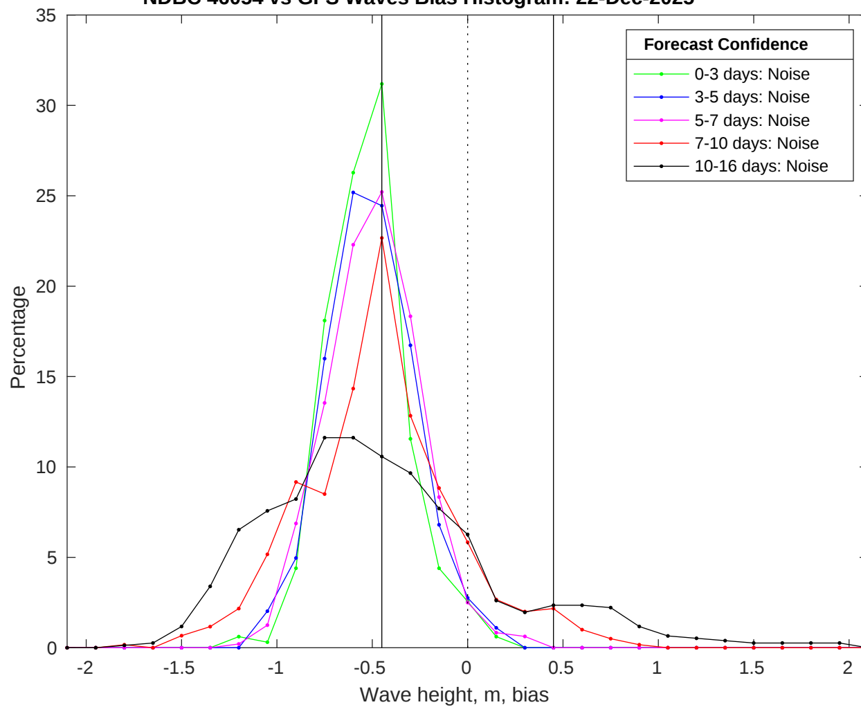
NDBC 46054 vs GFS Waves Bias Histogram: 22-Dec-2025
