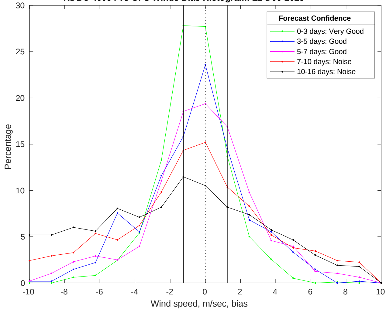
NDBC 46054 vs GFS Winds Bias Histogram: 22-Dec-2025
