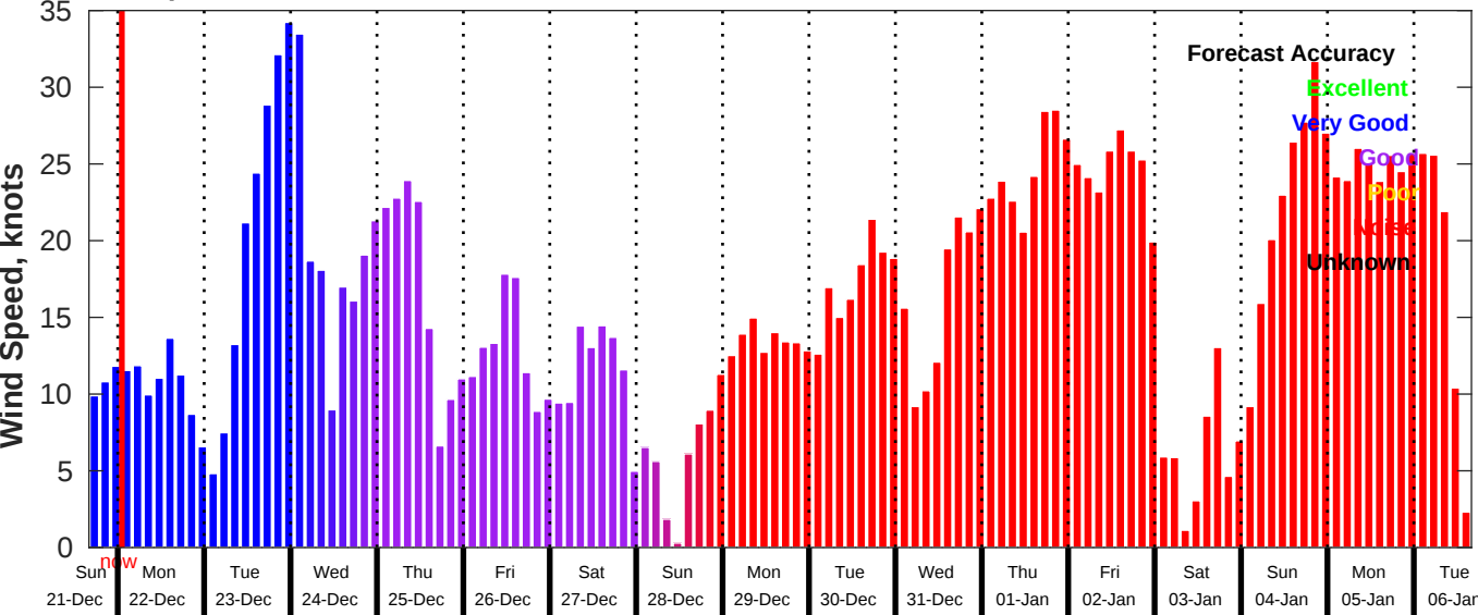
GFS Wind Speed Forecast for NDBC 46054 from 21-Dec-2025 16:00:00 to 06-Jan-2026 16:00:00
