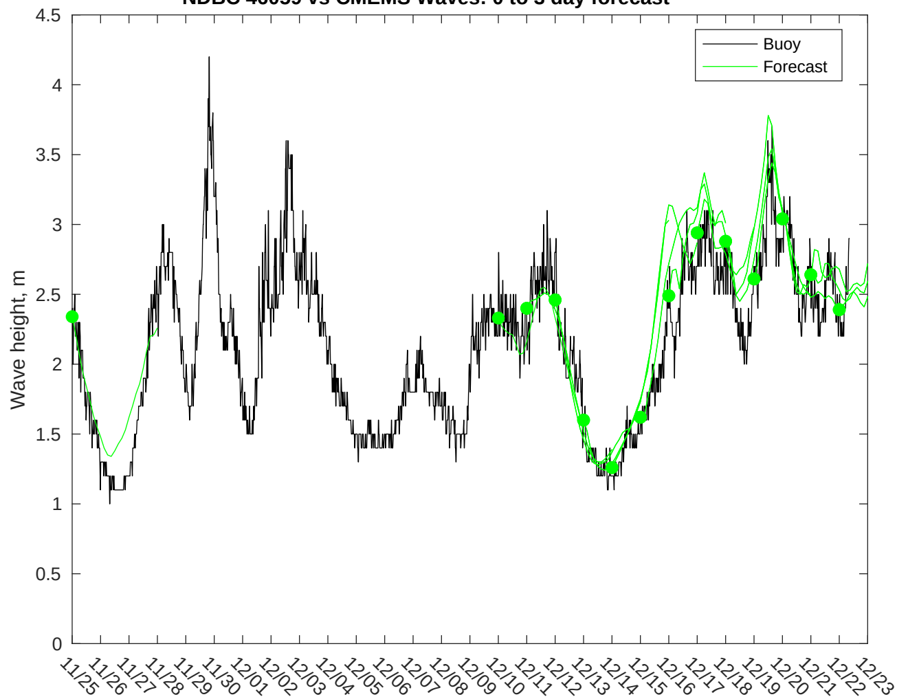
NDBC 46059 vs CMEMS Waves: 0 to 3 day forecast
