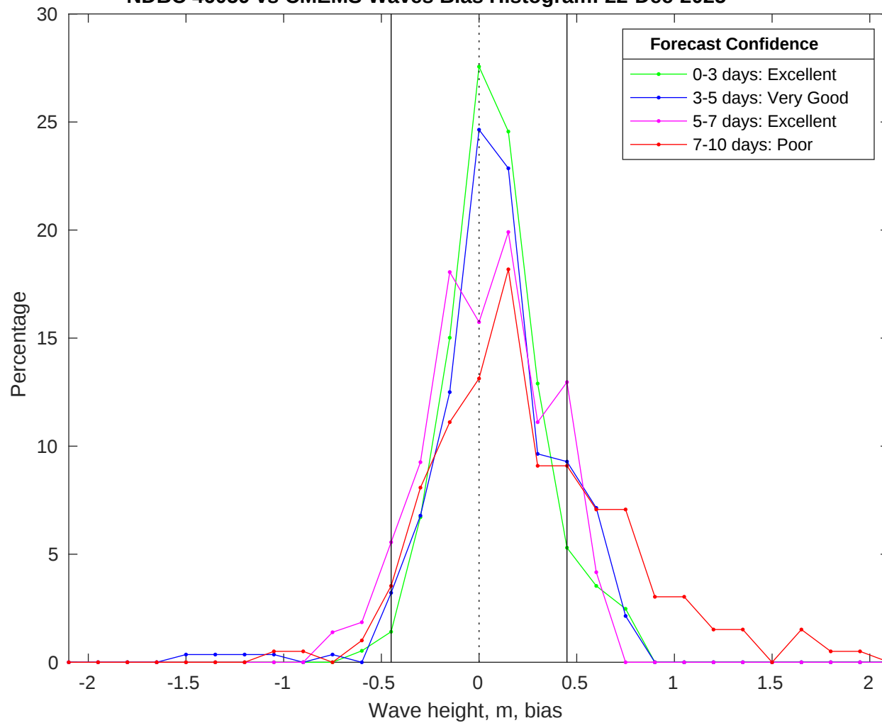
NDBC 46059 vs CMEMS Waves Bias Histogram: 22-Dec-2025
