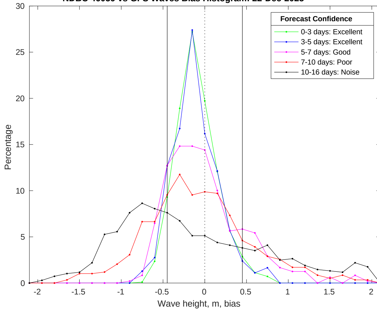
NDBC 46059 vs GFS Waves Bias Histogram: 22-Dec-2025
