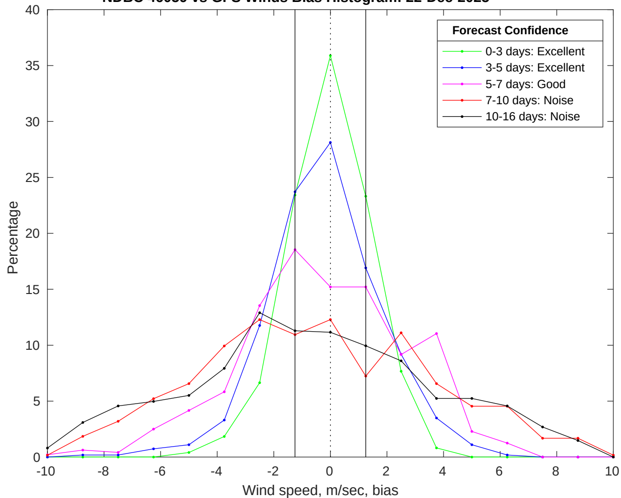
NDBC 46059 vs GFS Winds Bias Histogram: 22-Dec-2025
