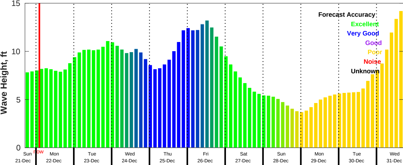
CMEMS Wave Forecast for NDBC 46059 from 21-Dec-2025 17:00:00 to 31-Dec-2025 17:00:00
