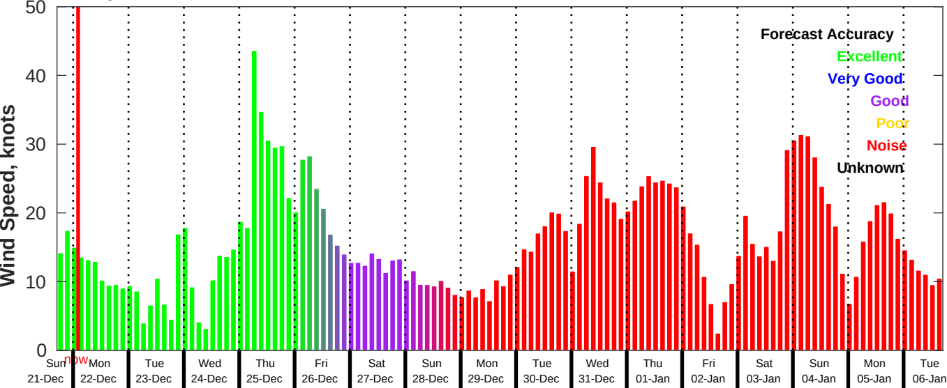
GFS Wind Speed Forecast for NDBC 46059 from 21-Dec-2025 17:00:00 to 06-Jan-2026 17:00:00
