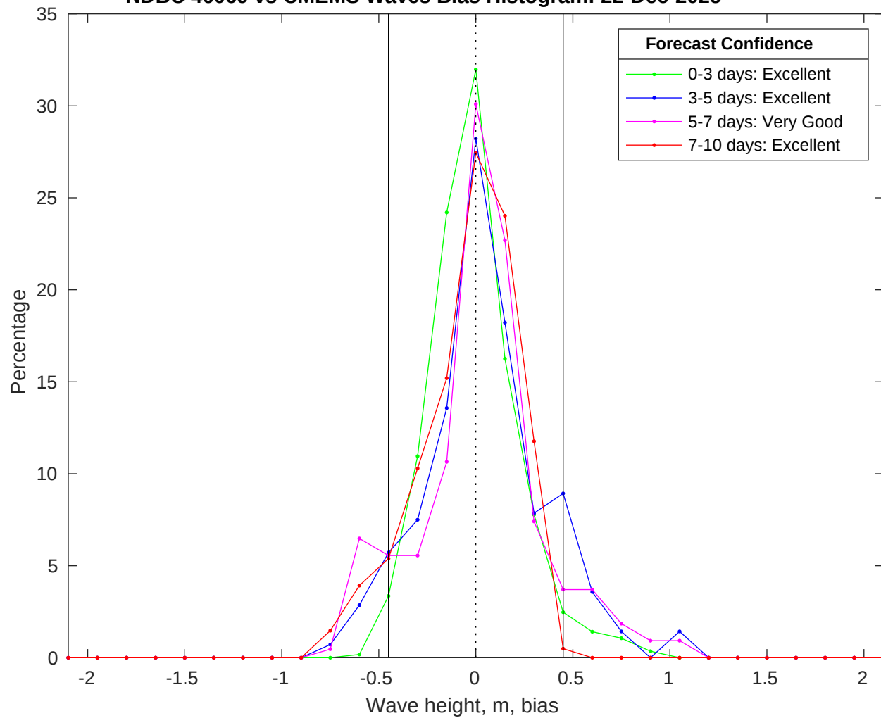
NDBC 46069 vs CMEMS Waves Bias Histogram: 22-Dec-2025
