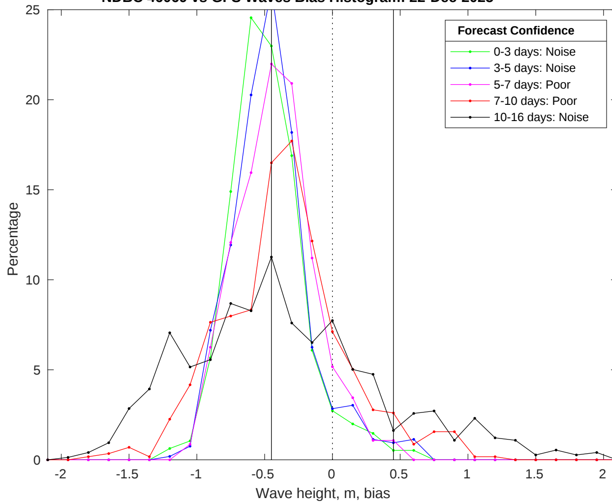
NDBC 46069 vs GFS Waves Bias Histogram: 22-Dec-2025
