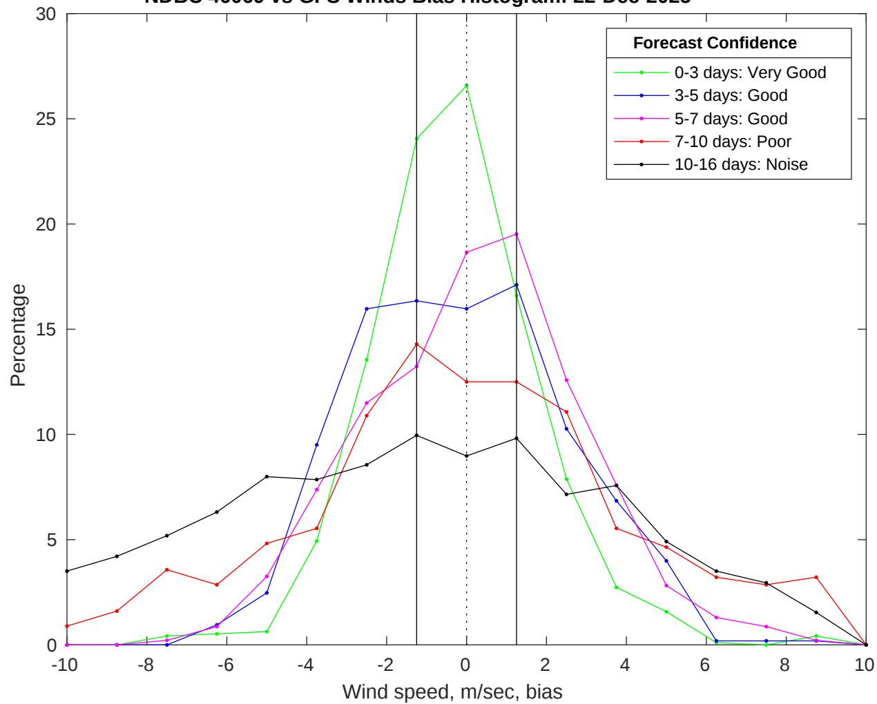
NDBC 46069 vs GFS Winds Bias Histogram: 22-Dec-2025
