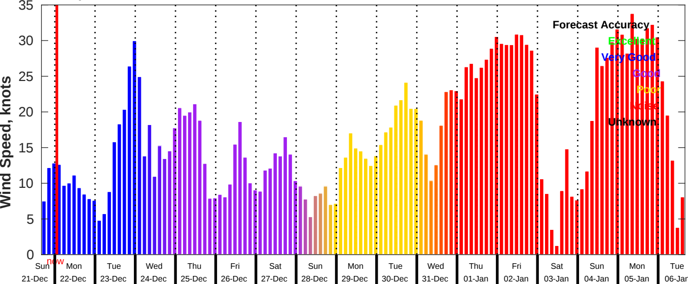
GFS Wind Speed Forecast for NDBC 46069 from 21-Dec-2025 16:00:00 to 06-Jan-2026 16:00:00
