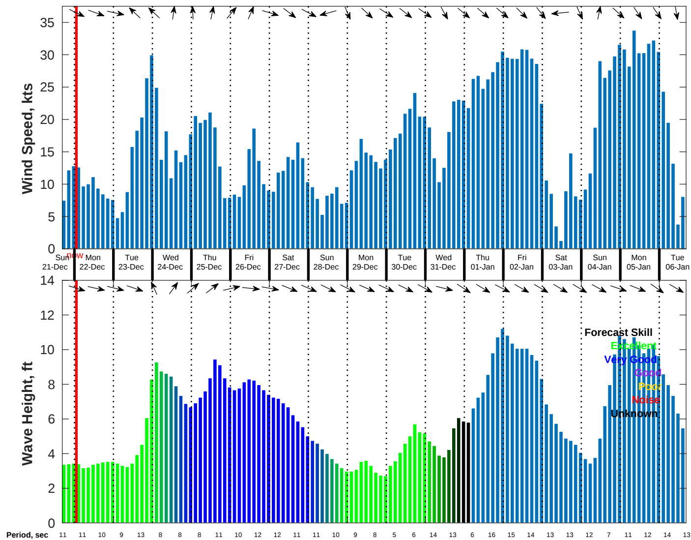
Wind & Wave Forecast for NDBC 46069 from 21-Dec-2025 16:00:00 to 06-Jan-2026 16:00:00
