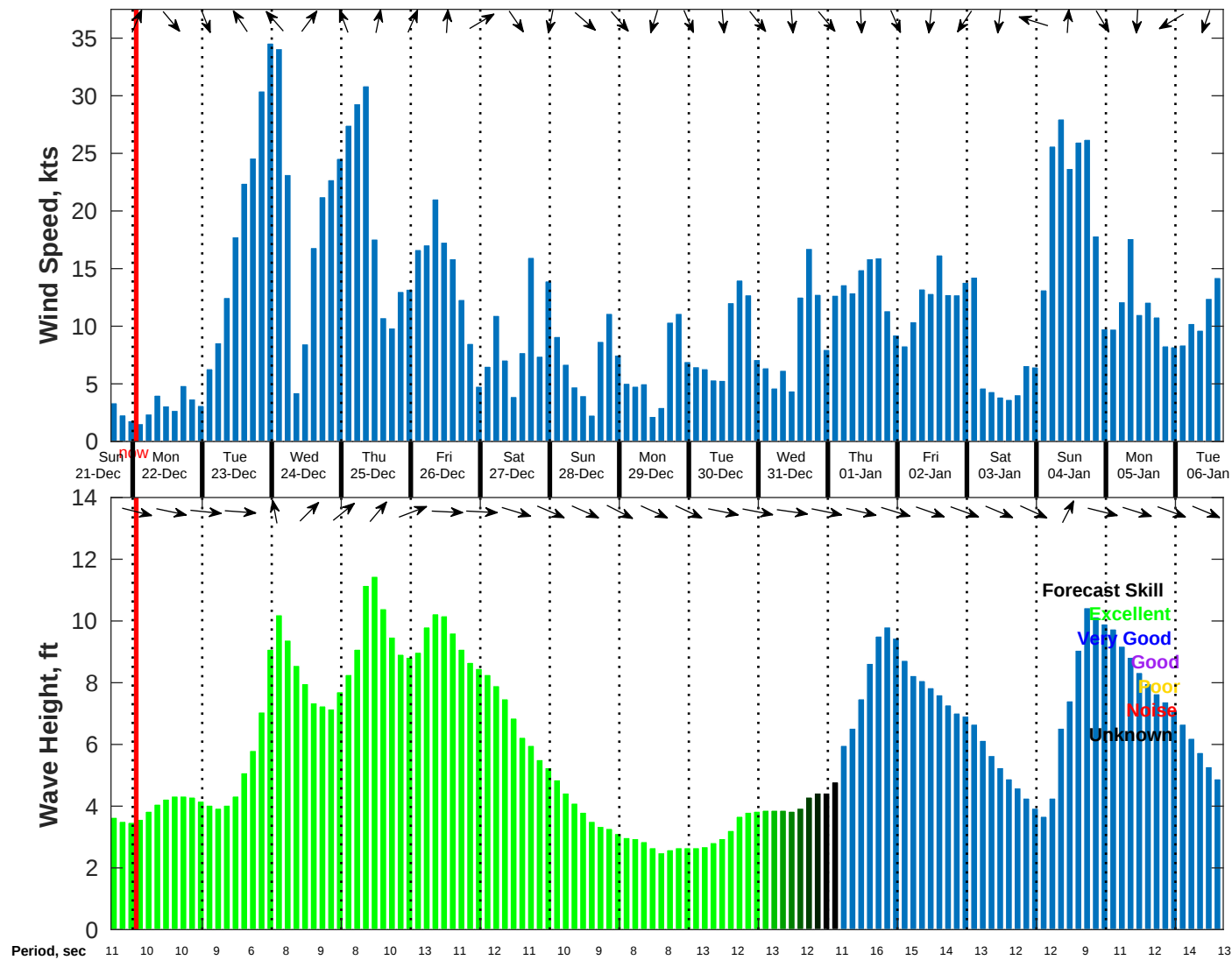
Wind & Wave Forecast for NDBC 46215 from 21-Dec-2025 16:00:00 to 06-Jan-2026 16:00:00
