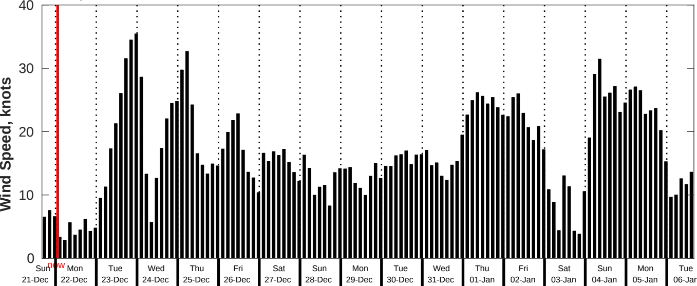
GFS Wind Speed Forecast for NDBC 46259 from 21-Dec-2025 16:00:00 to 06-Jan-2026 16:00:00
