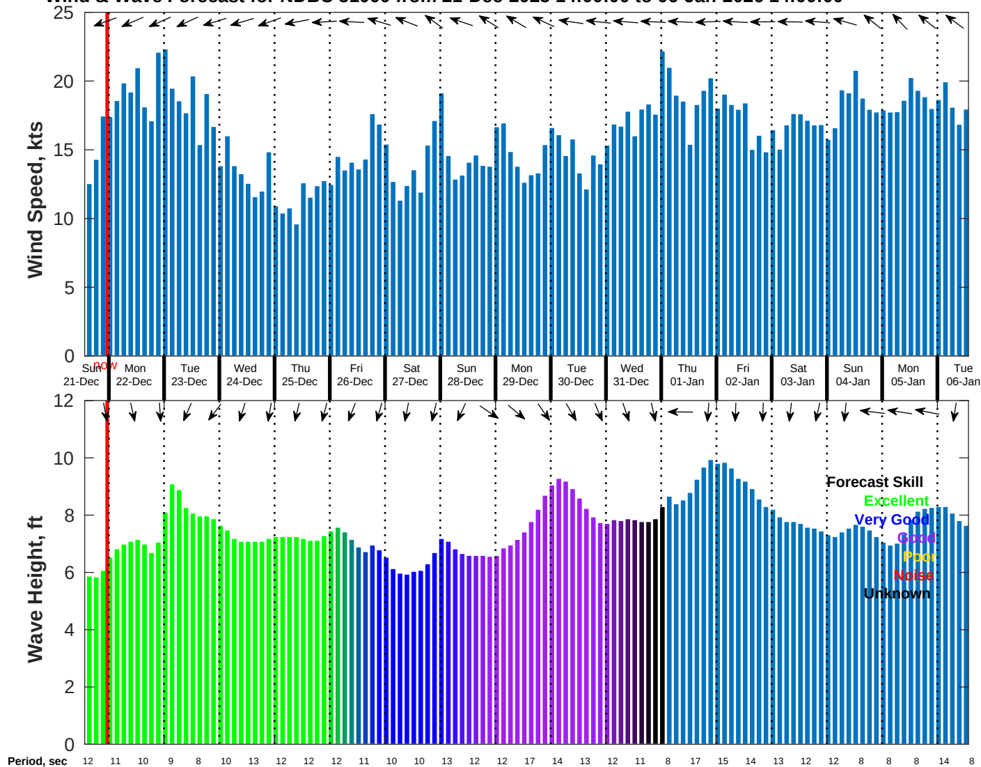
Wind & Wave Forecast for NDBC 51000 from 21-Dec-2025 14:00:00 to 06-Jan-2026 14:00:00
