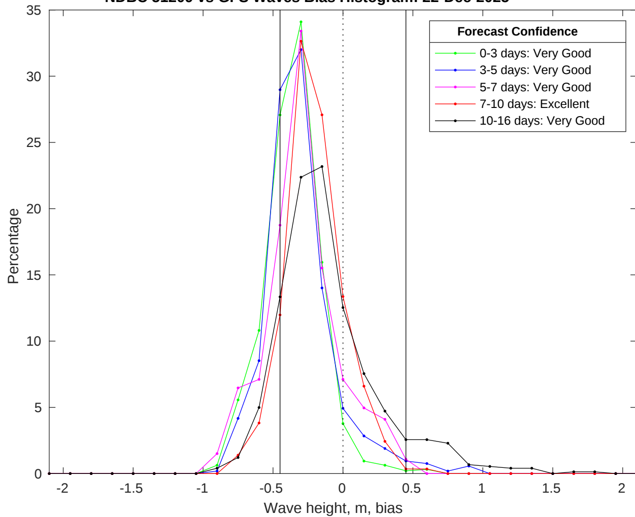
NDBC 51209 vs GFS Waves Bias Histogram: 22-Dec-2025
