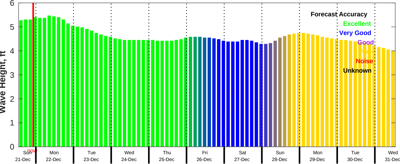
CMEMS Wave Forecast for NDBC 51209 from 21-Dec-2025 13:00:00 to 31-Dec-2025 13:00:00
