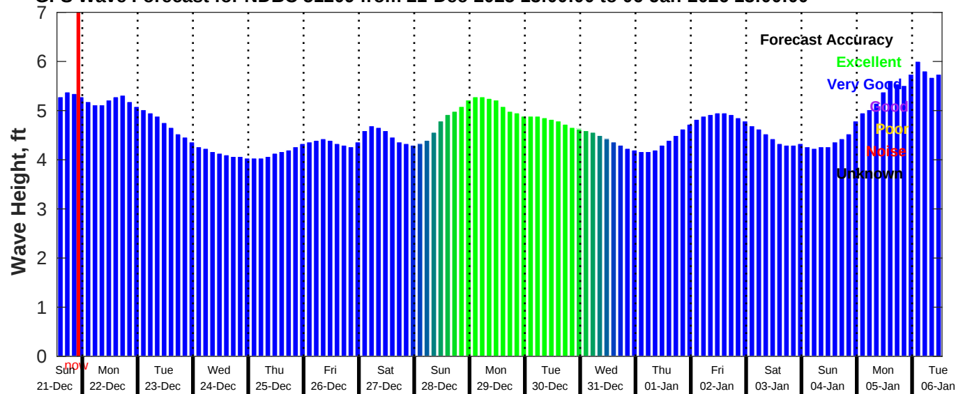
GFS Wave Forecast for NDBC 51209 from 21-Dec-2025 13:00:00 to 06-Jan-2026 13:00:00
