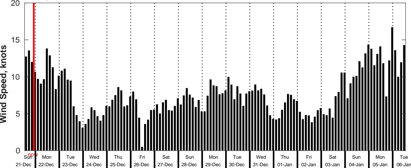
GFS Wind Speed Forecast for NDBC 51209 from 21-Dec-2025 13:00:00 to 06-Jan-2026 13:00:00
