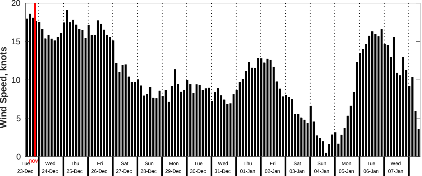
GFS Wind Speed Forecast for NDBC 52211 from 22-Dec-2025 11:00:00 to 07-Jan-2026 11:00:00
