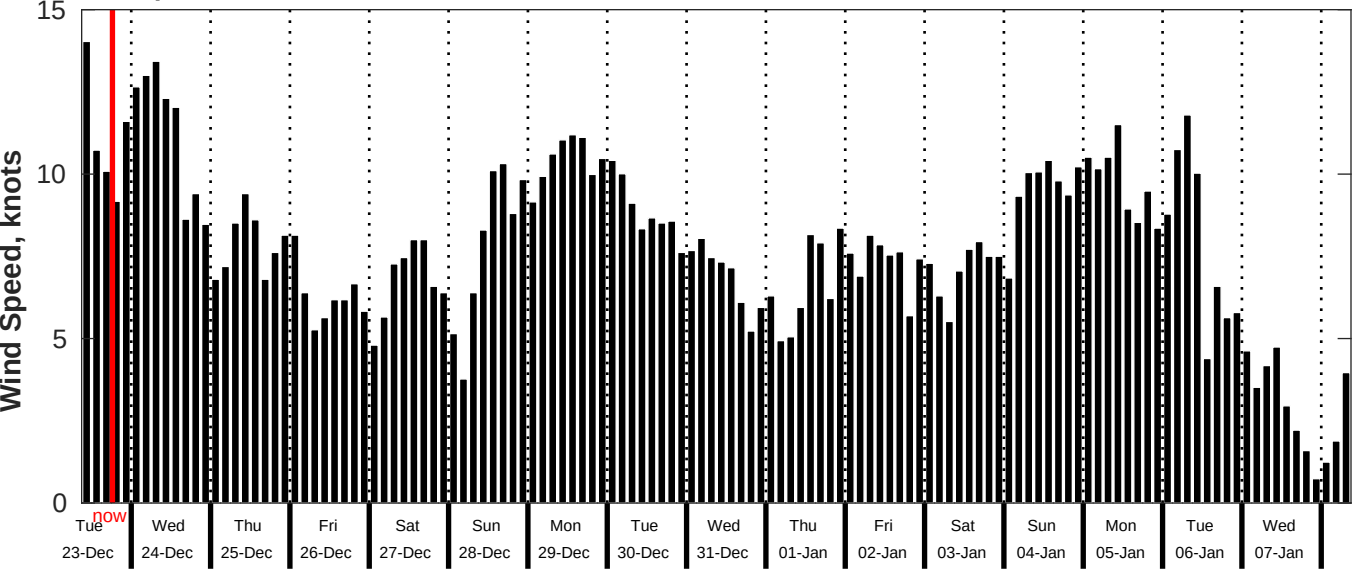
GFS Wind Speed Forecast for NDBC 52212 from 22-Dec-2025 09:00:00 to 07-Jan-2026 09:00:00
