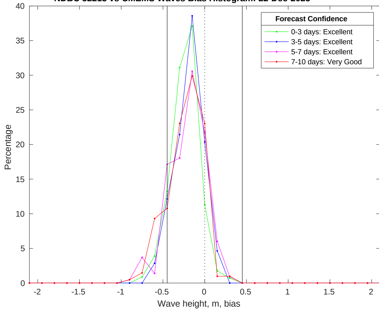
NDBC 52213 vs CMEMS Waves Bias Histogram: 22-Dec-2025
