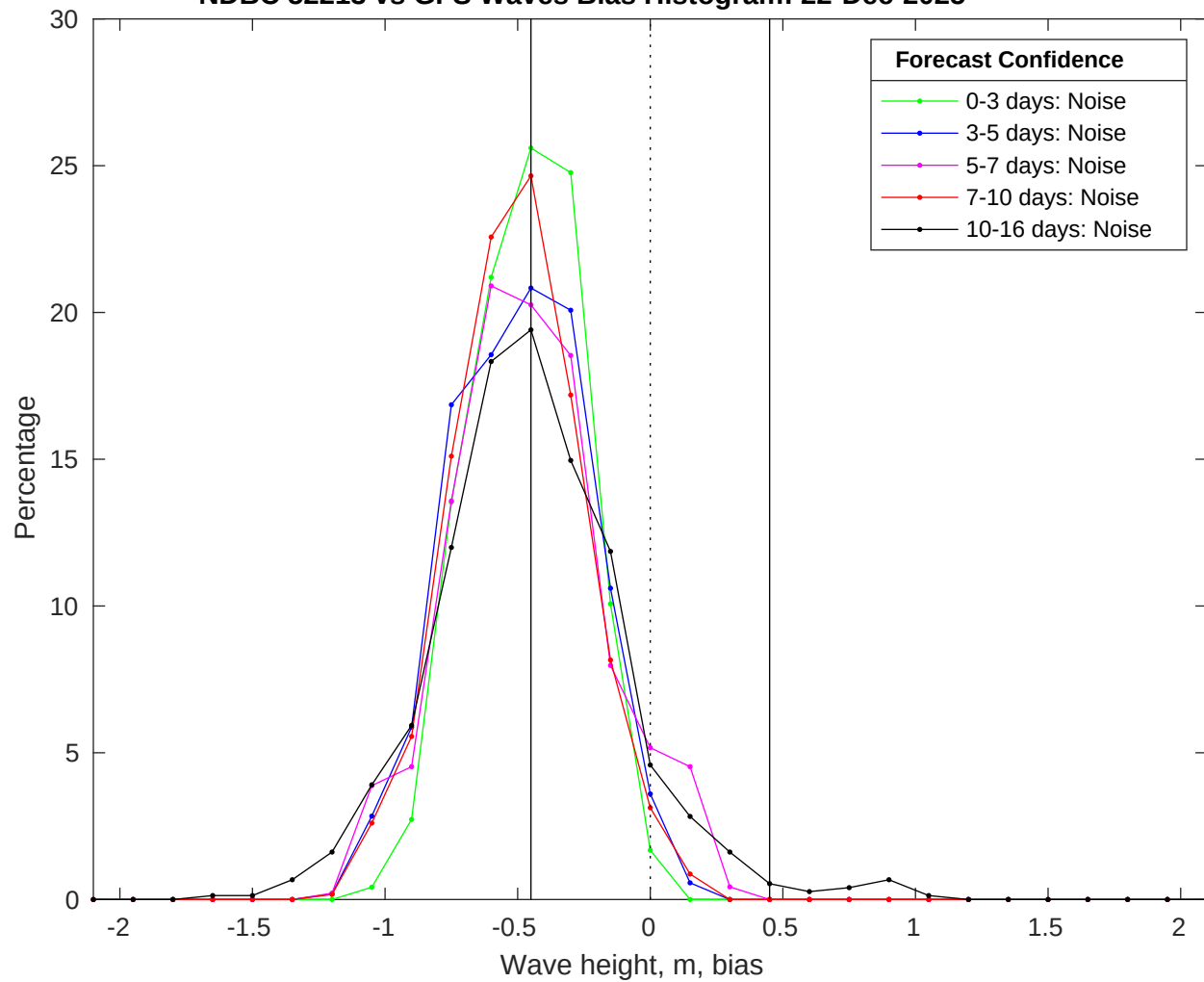
NDBC 52213 vs GFS Waves Bias Histogram: 22-Dec-2025
