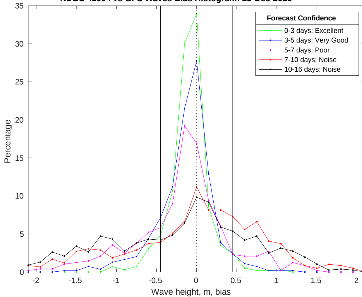
NDBC 41004 vs GFS Waves Bias Histogram: 23-Dec-2025
