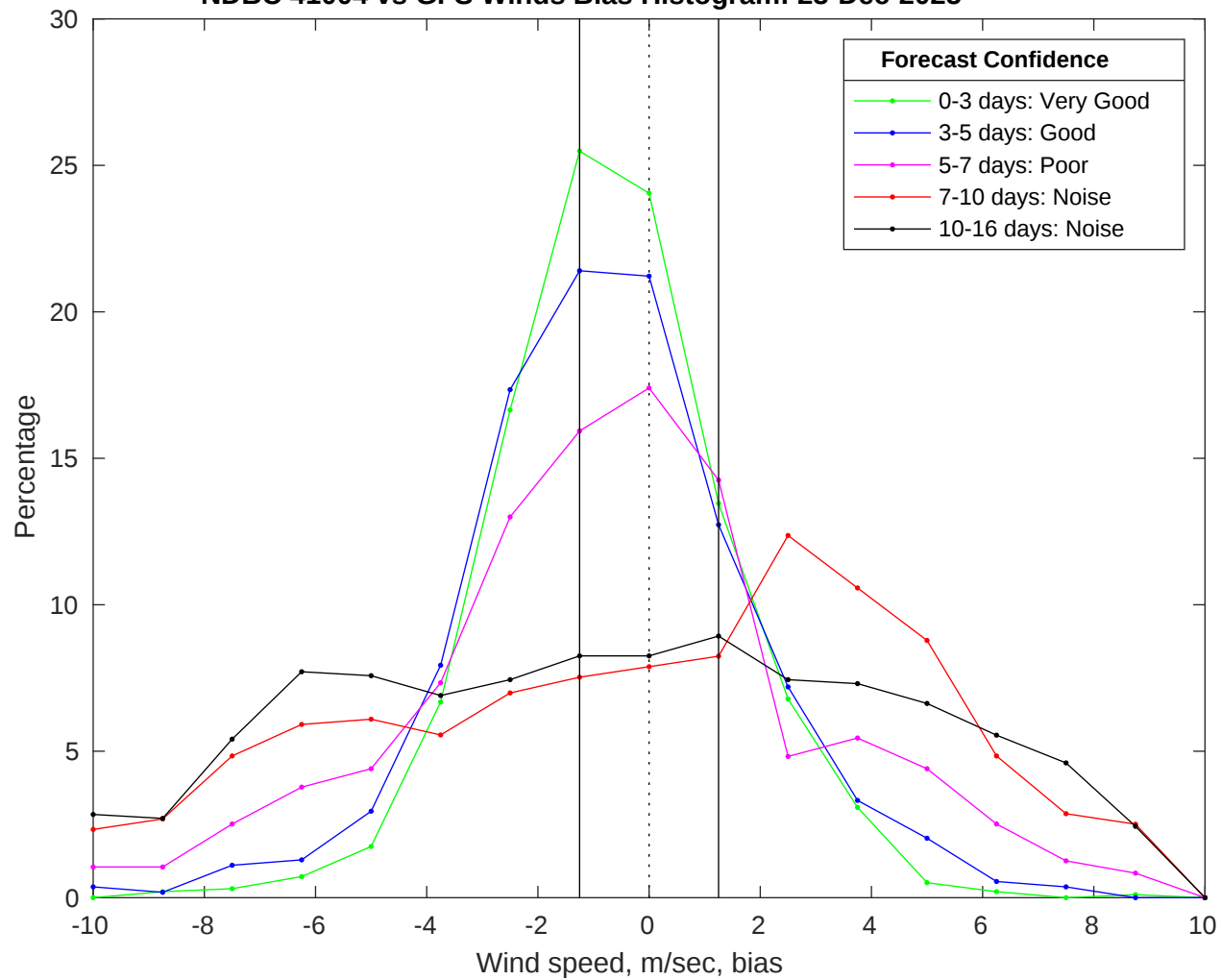
NDBC 41004 vs GFS Winds Bias Histogram: 23-Dec-2025
