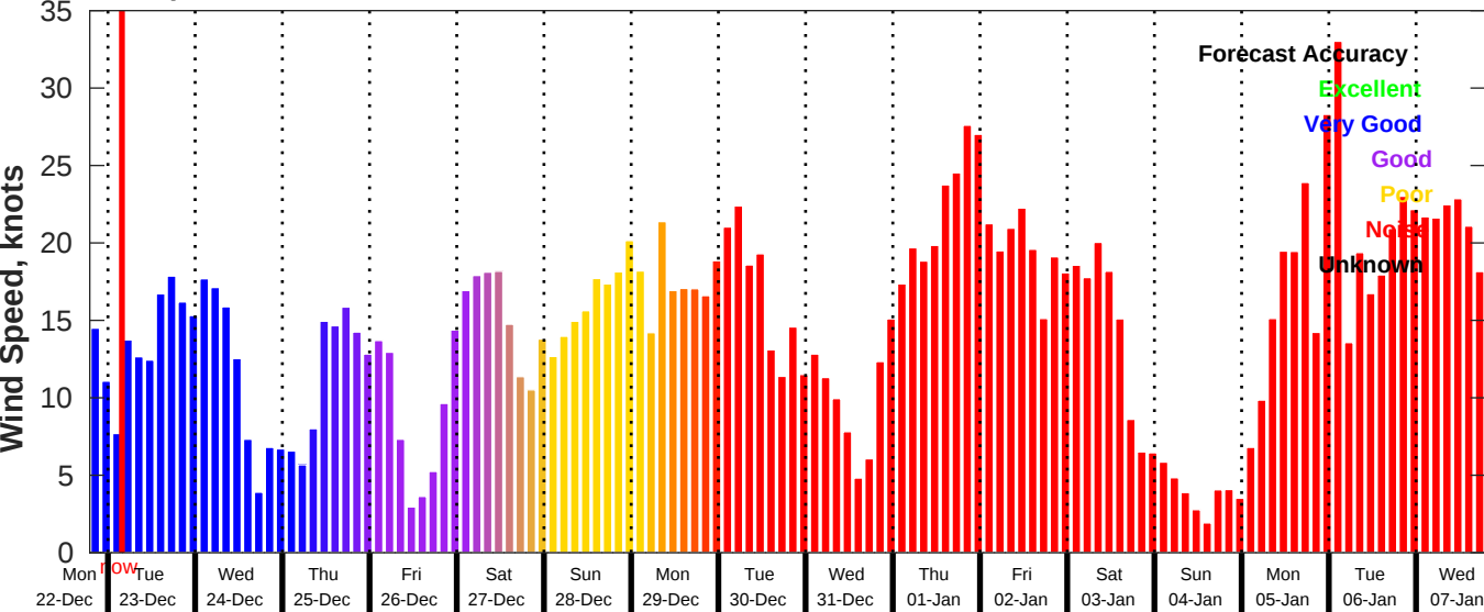
GFS Wind Speed Forecast for NDBC 41004 from 22-Dec-2025 19:00:00 to 07-Jan-2026 19:00:00
