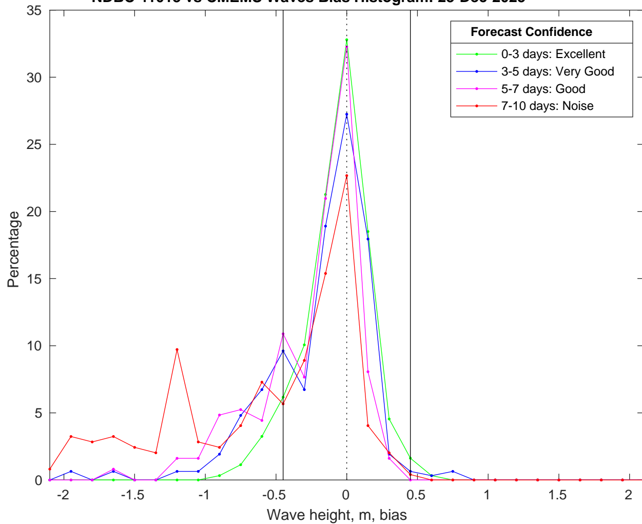
NDBC 41013 vs CMEMS Waves Bias Histogram: 23-Dec-2025
