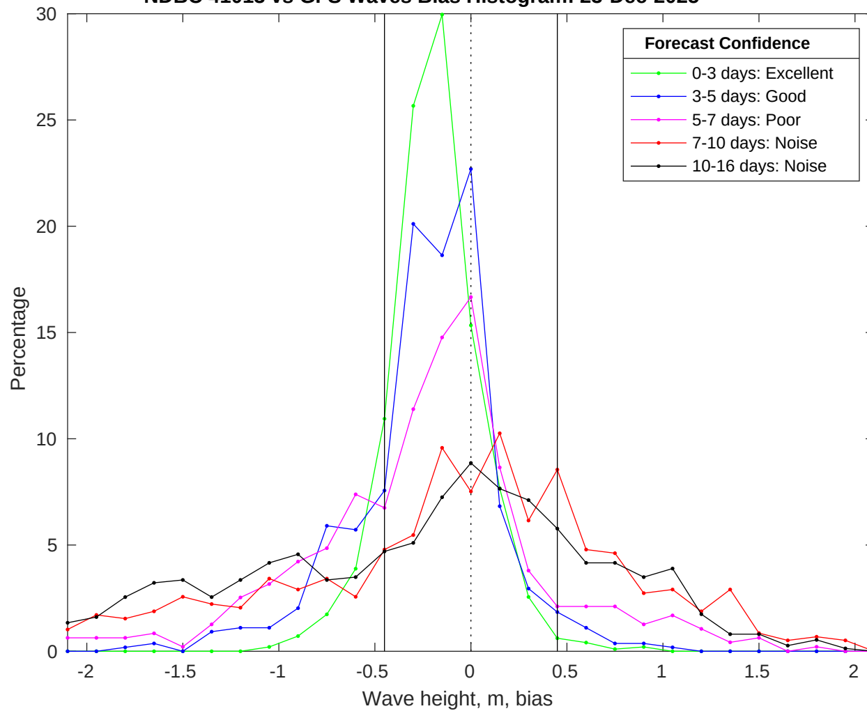
NDBC 41013 vs GFS Waves Bias Histogram: 23-Dec-2025
